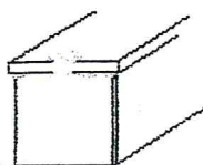
Figure (C) Chipped area of Ivory, as well as reservoir below lip of keytop have been filled with repair material. (Shown in grey)
